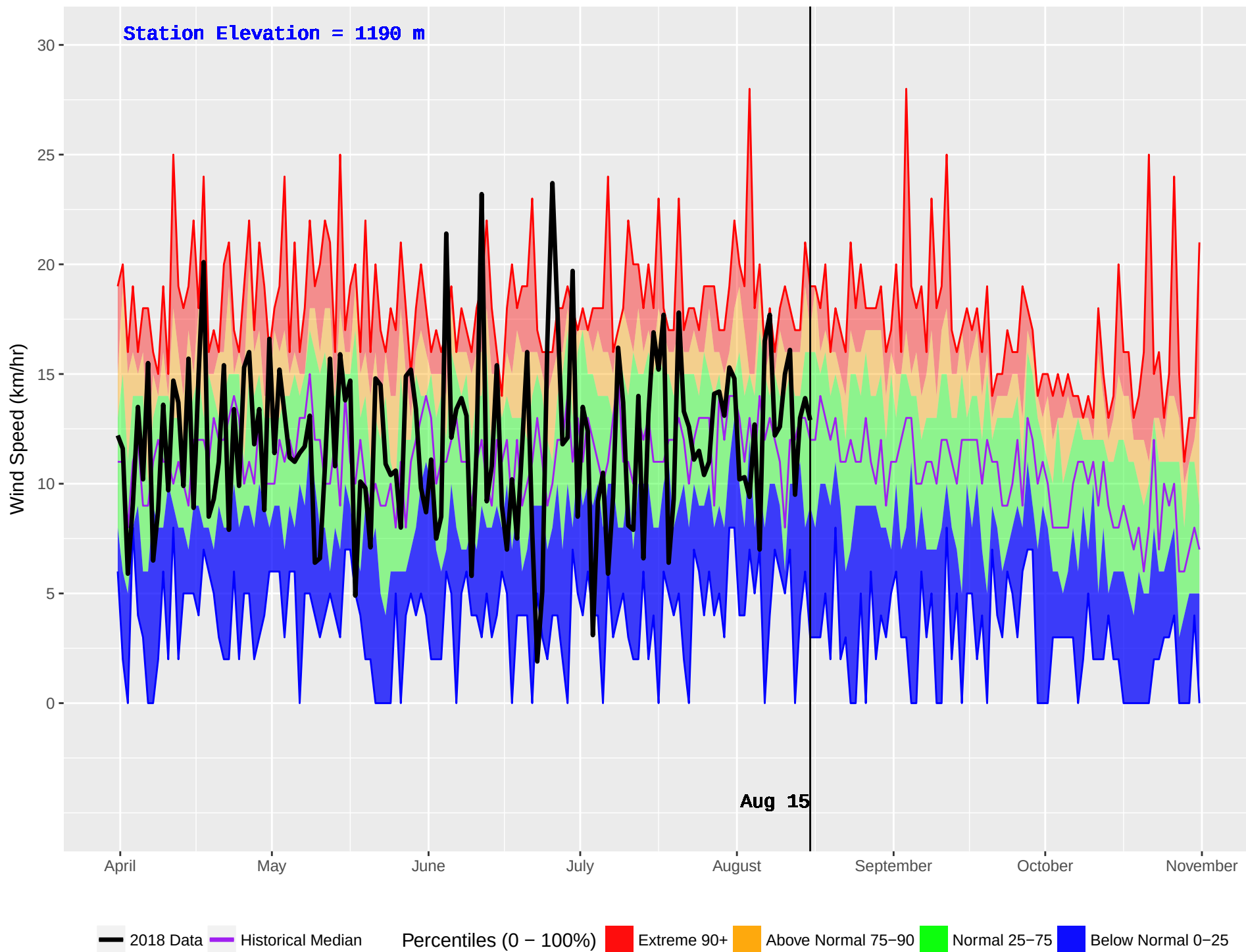
EMILY CREEK (425) : Historical (2002–2016) and Current (2018) Daily Wind Speed
