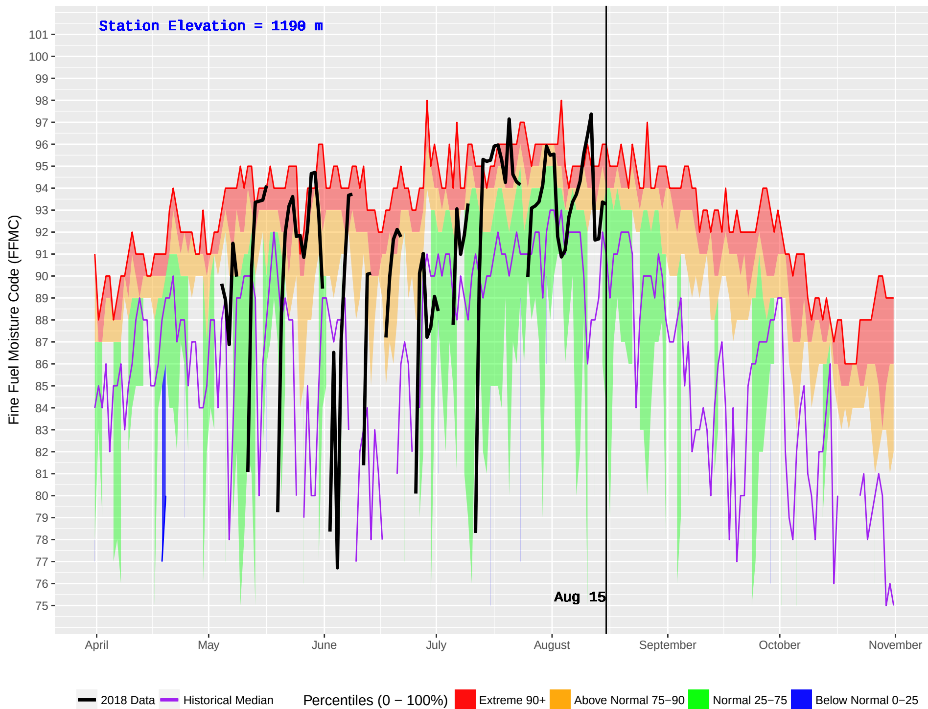
EMILY CREEK (425) : Historical (2002–2016) and Current (2018) Daily Fine Fuel Moisture Code (FFMC)
